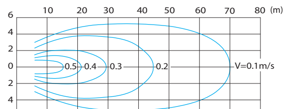
MA5/12-620-480
