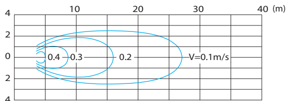
MA1.5/8-400-740
