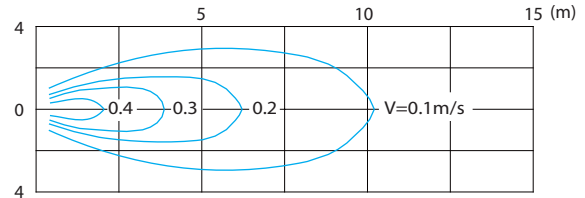
MA0.55/4-220-1400
